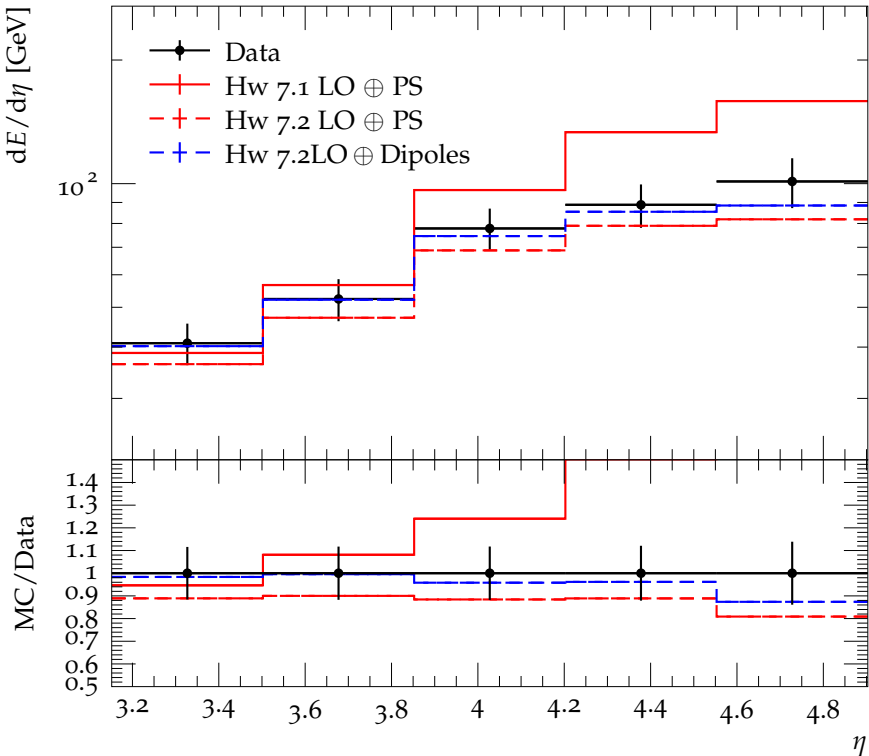
Energy flow in MB events, \sqrt{s} = 0.9 TeV
