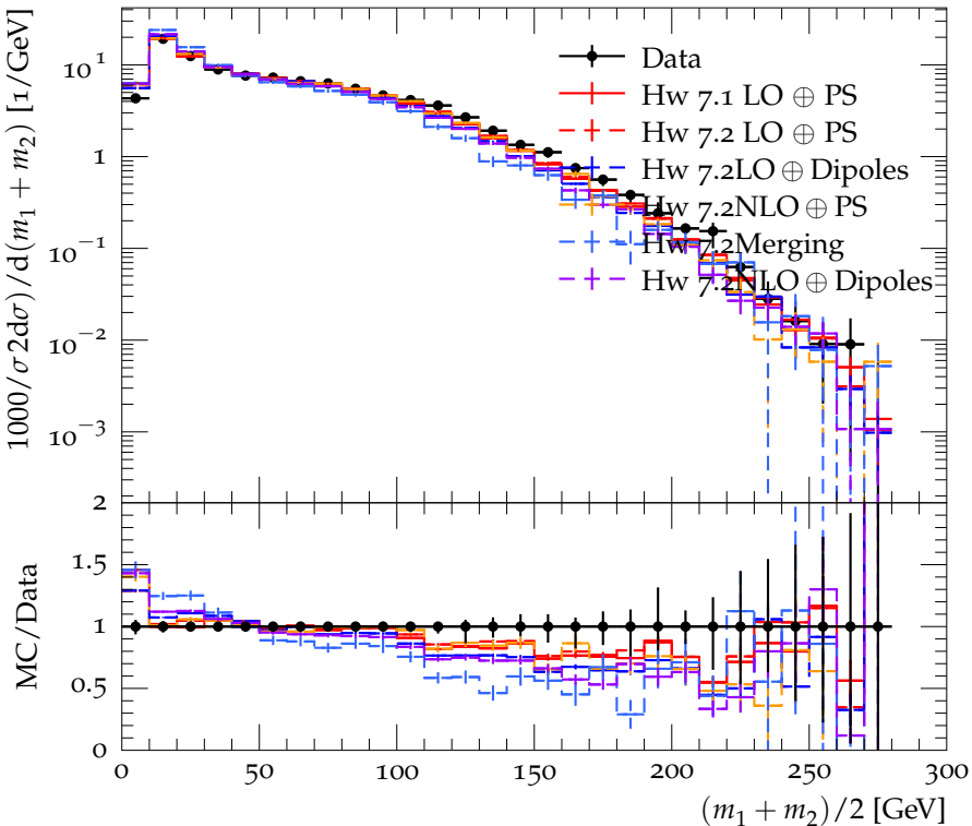
Pruned AK7 dijets, (p_T^1 + p_T^2)/2 = 600\text{--}800 GeV
