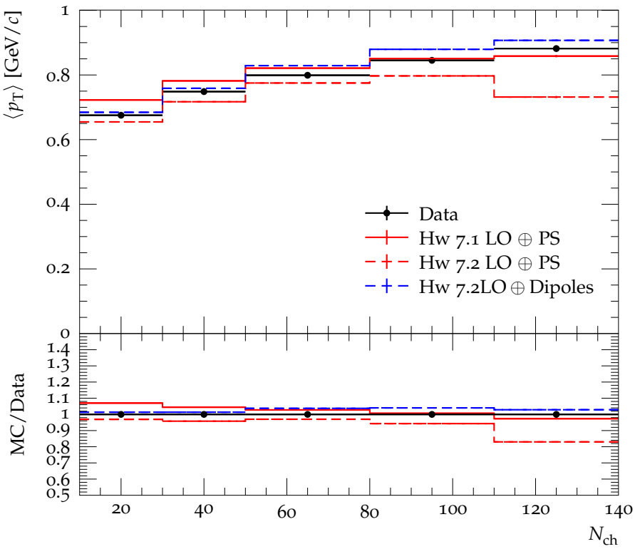
Mean p_T , all charged particles
