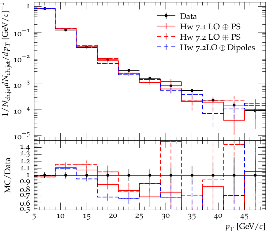
Jet T spectrum, |\eta^{\text{ch,jet}}| < 1.9, 80 < N_{\text{ch}} \leq 110
