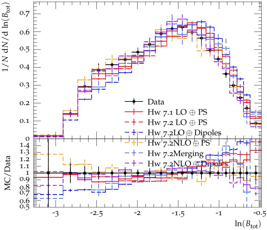
Jet broadening for 110 < p_{T,1} < 170 and |\eta| < 2.4
