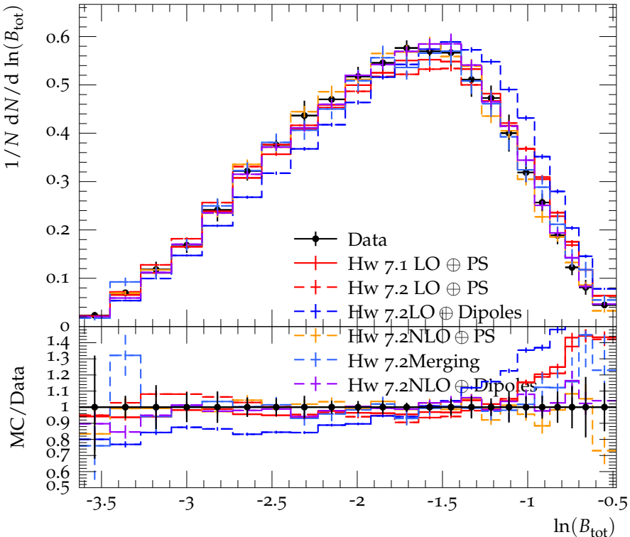
Jet broadening for 250 < p_{T,1} < 320 and |\eta| < 2.4
