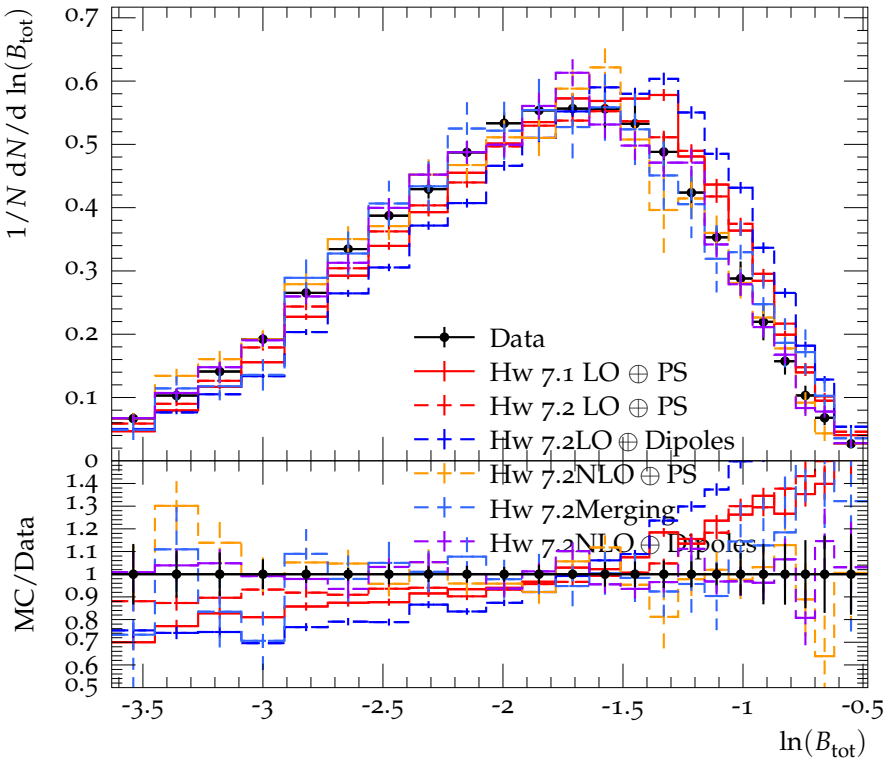
Jet broadening for 320 < p_{T,1} < 390 and |\eta| < 2.4
