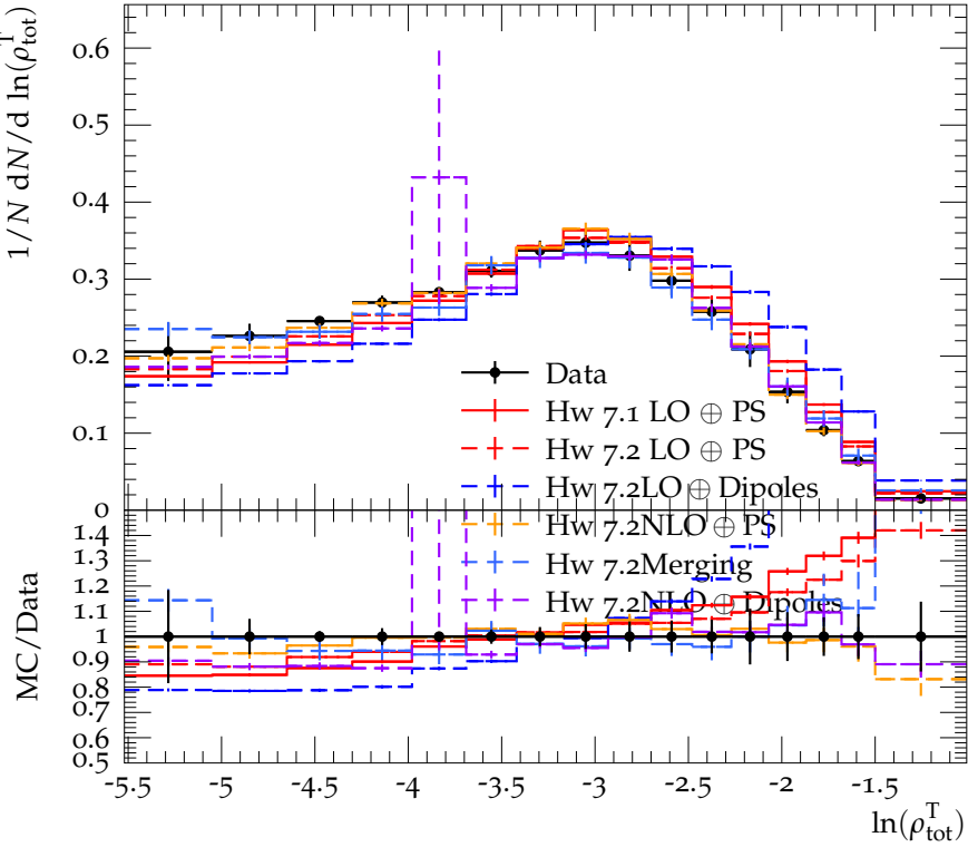
Total transverse jet mass for p_{T,1} > 390 and |\eta| < 2.4
