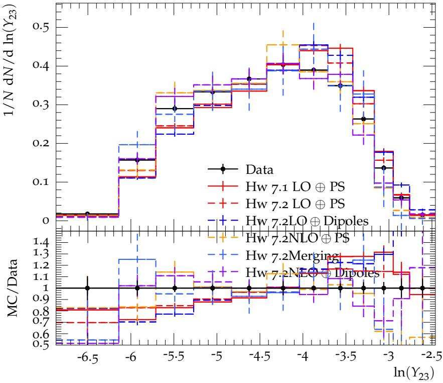
Third-jet resolution parameter for 170 < p_{T,1} < 250 and |\eta| < 2.4
