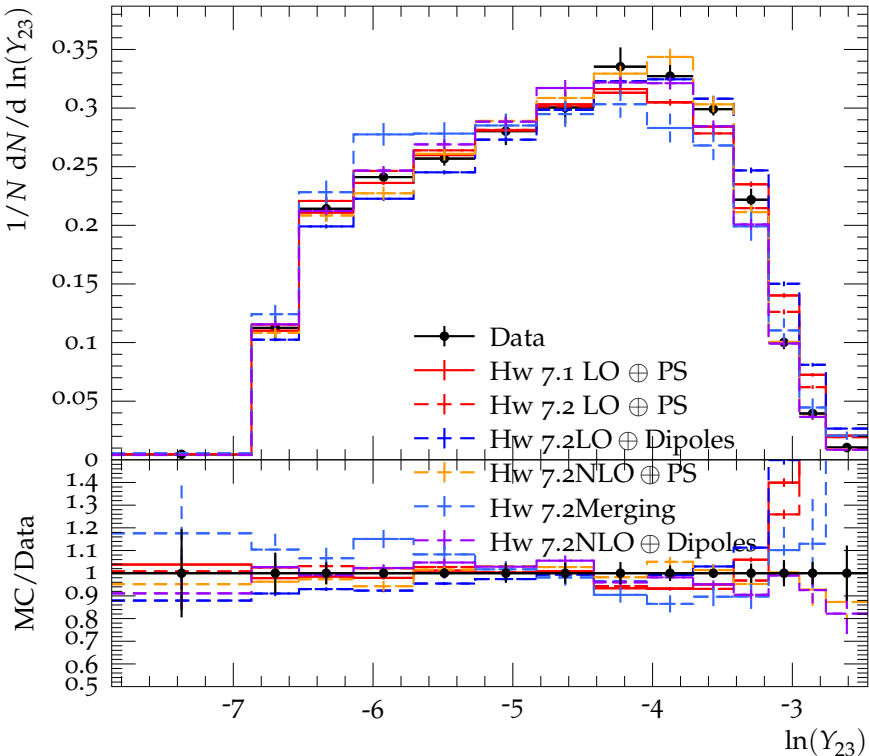
Third-jet resolution parameter for 250 < p_{T,1} < 320 and |\eta| < 2.4
