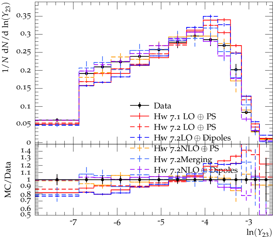
Third-jet resolution parameter for 320 < p_{T,1} < 390 and |\eta| < 2.4
