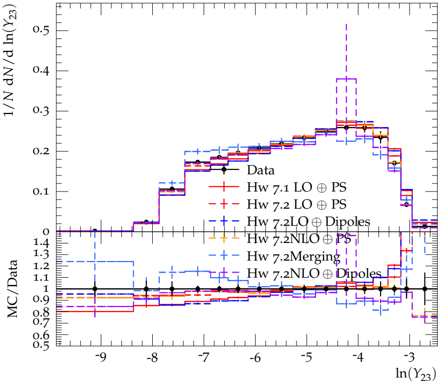
Third-jet resolution parameter for p_{T,1} > 390 and |\eta| < 2.4
