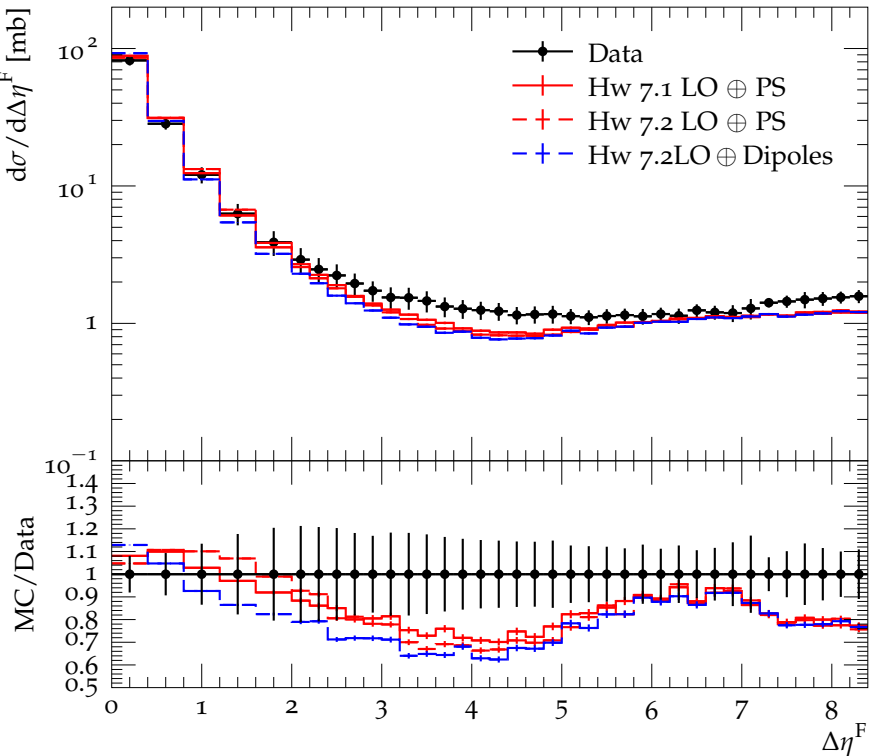
Rapidity gap size in \eta starting from \eta = \pm 4.7 , p_T > 200 MeV
