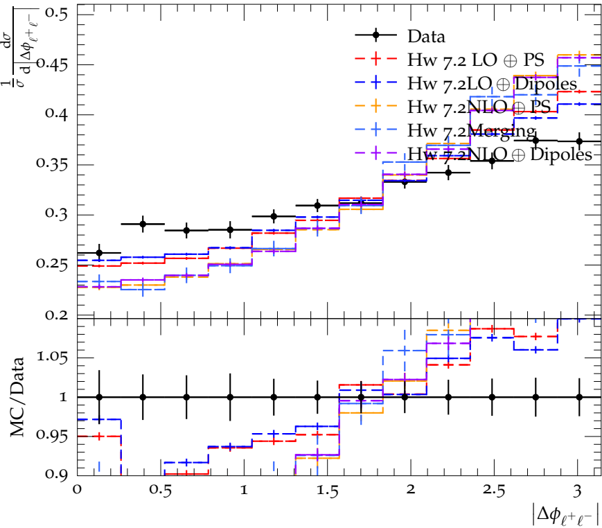
CMS, 8 TeV, t\bar{t} dilepton, parton-level. Rivet particle-level, e\mu only.
