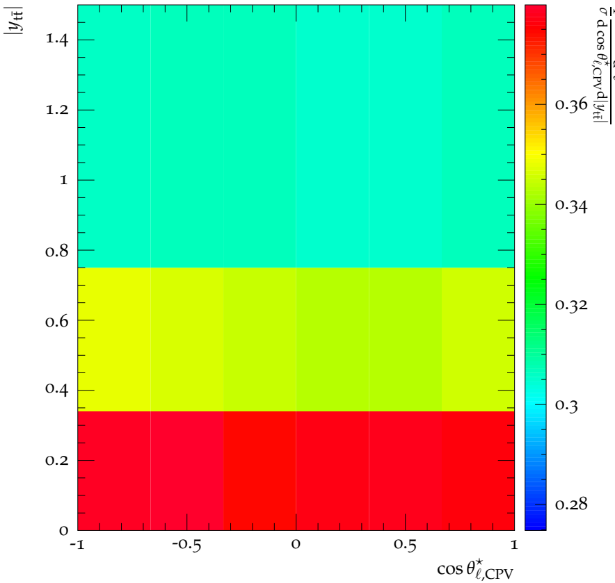
CMS, 8 TeV, t\bar{t} dilepton channel, Harton Level Dipoles
