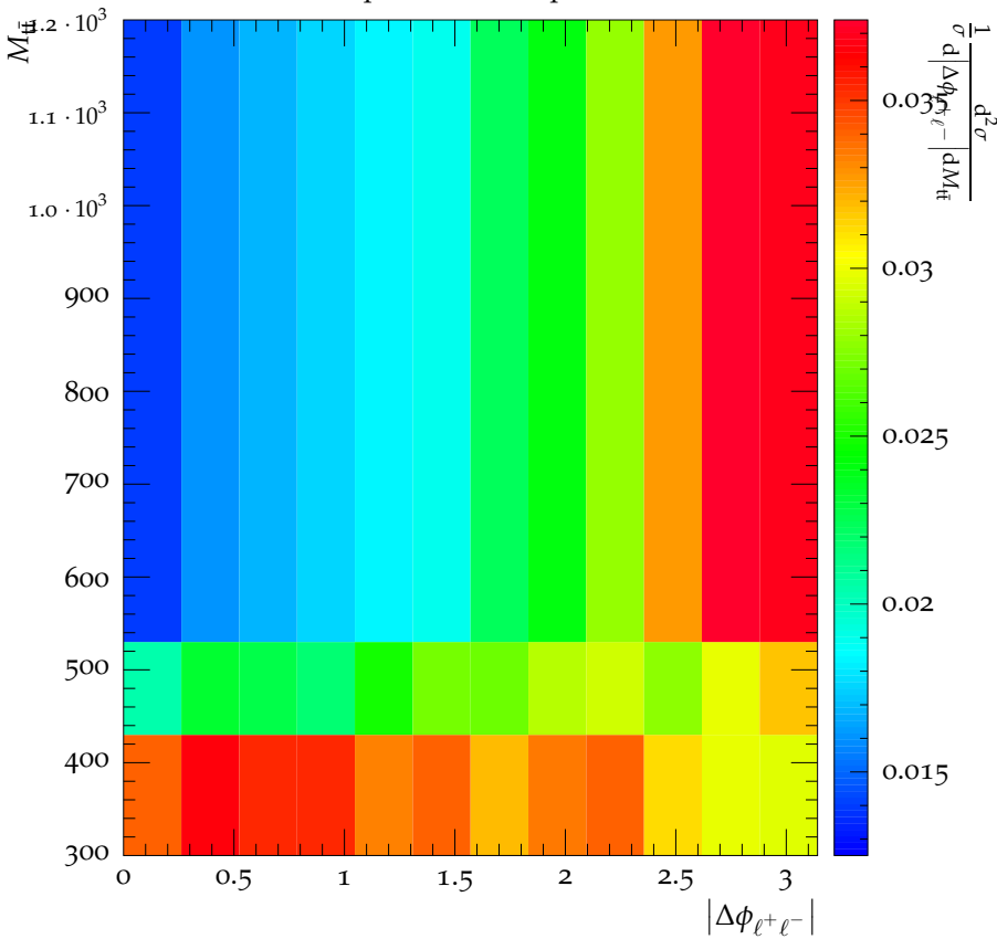
CMS, 8 TeV, t\bar{t} dilepton channel, parton-level
