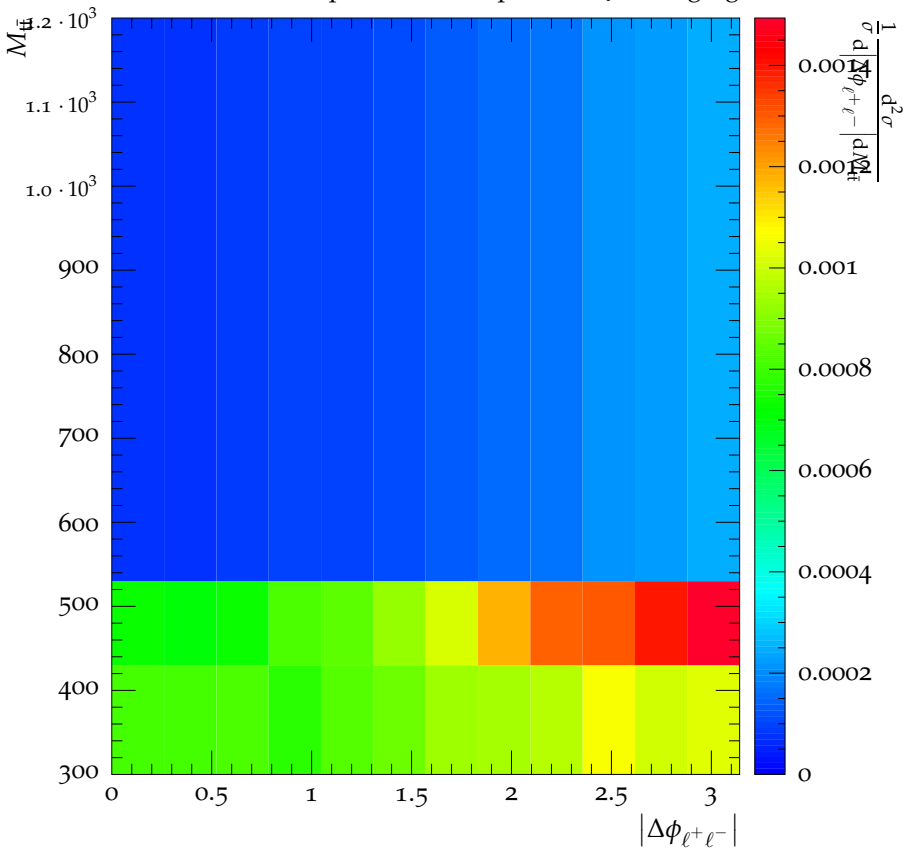
CMS, 8 TeV, t\bar{t} dilepton channel, parton-level \Delta\phi Merging
