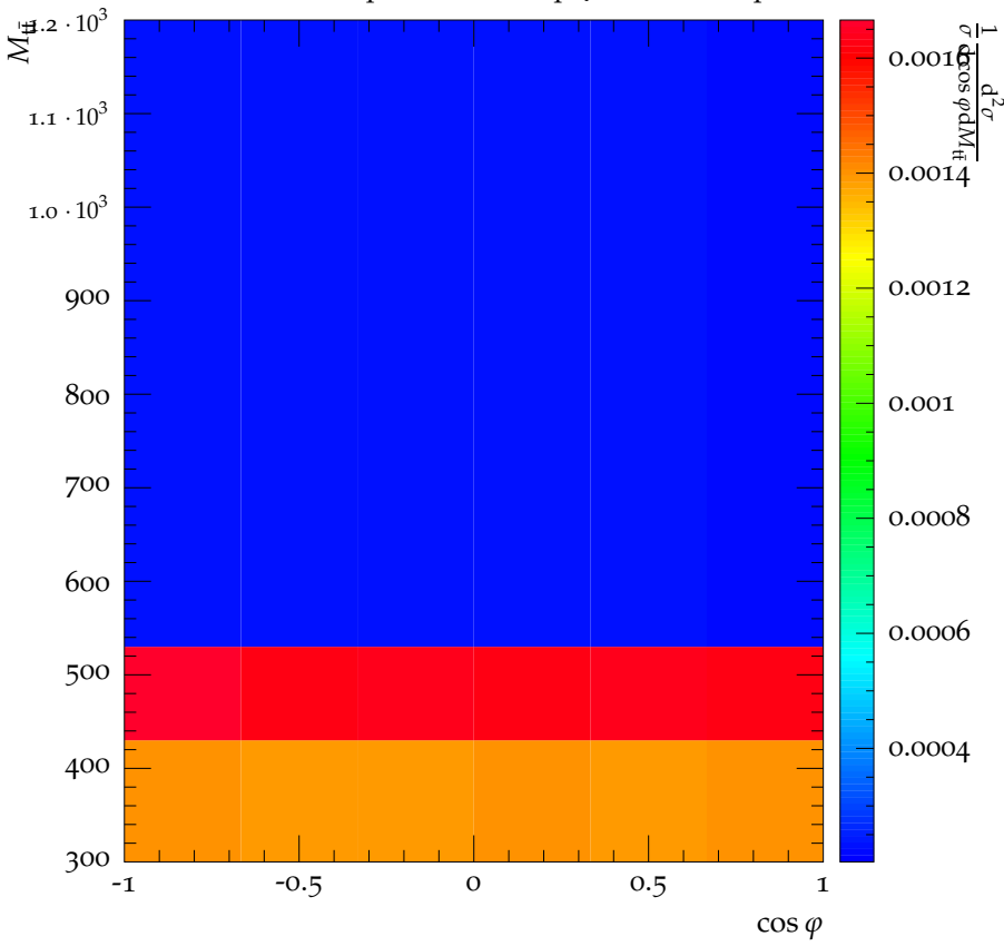
CMS, 8 TeV, t\bar{t} dilepton channel, H, \gamma to W Level-1 Dipoles
