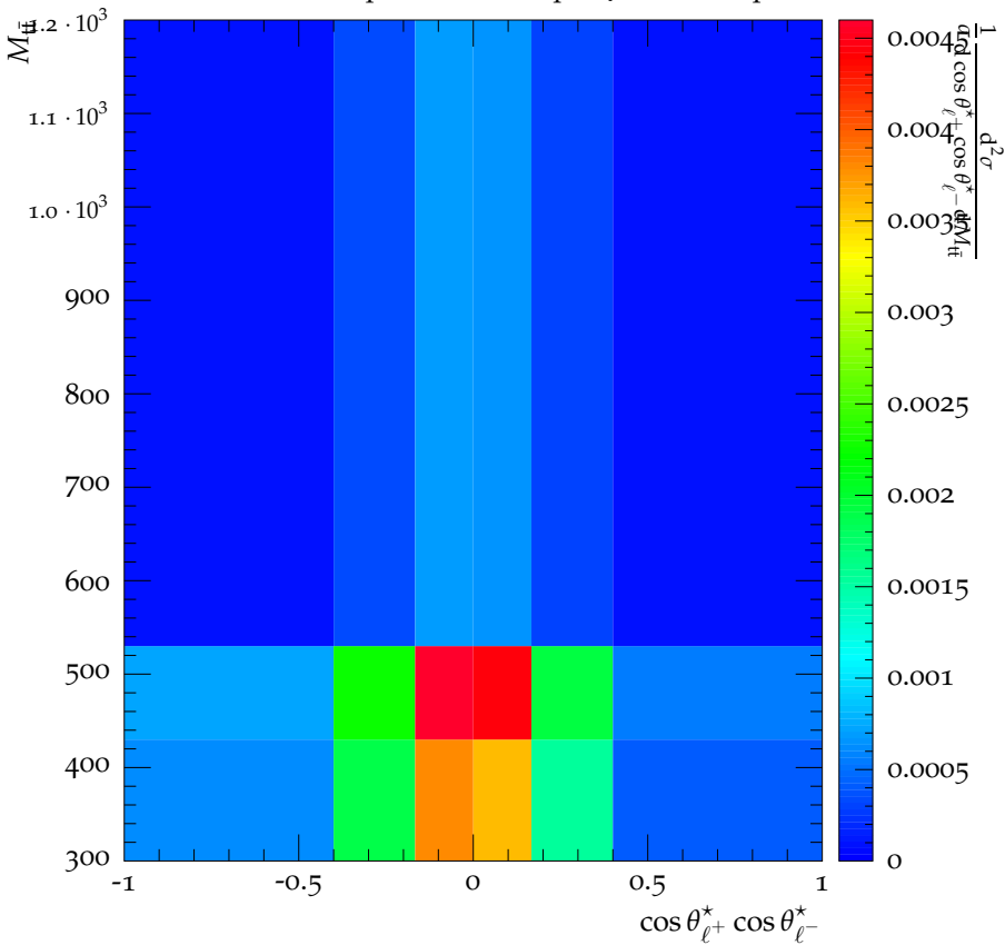
CMS, 8 TeV, t\bar{t} dilepton channel, \mu\tau Level Dipoles
