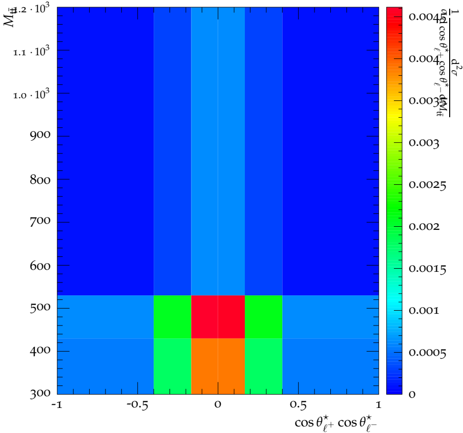
CMS, 8 TeV, t\bar{t} dilepton channel, Hvarion NLO Dipoles
