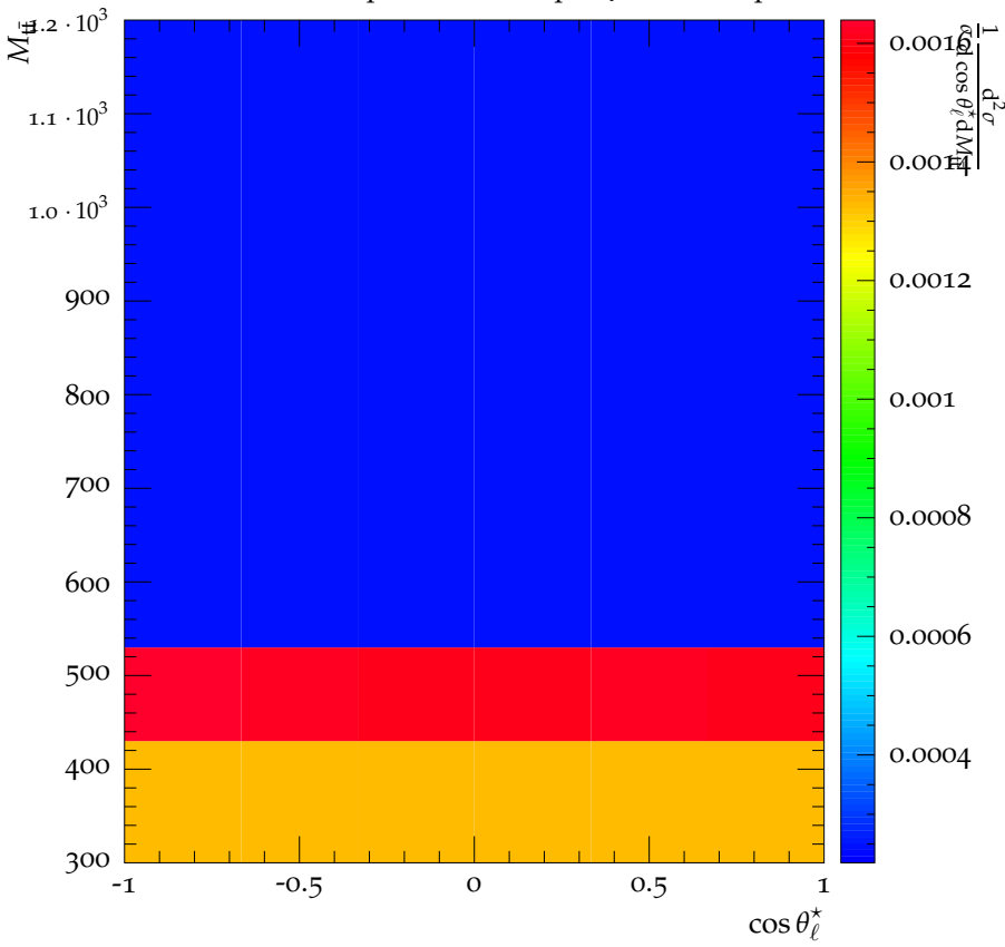
CMS, 8 TeV, t\bar{t} dilepton channel, \mu on Level-1 Dipoles
