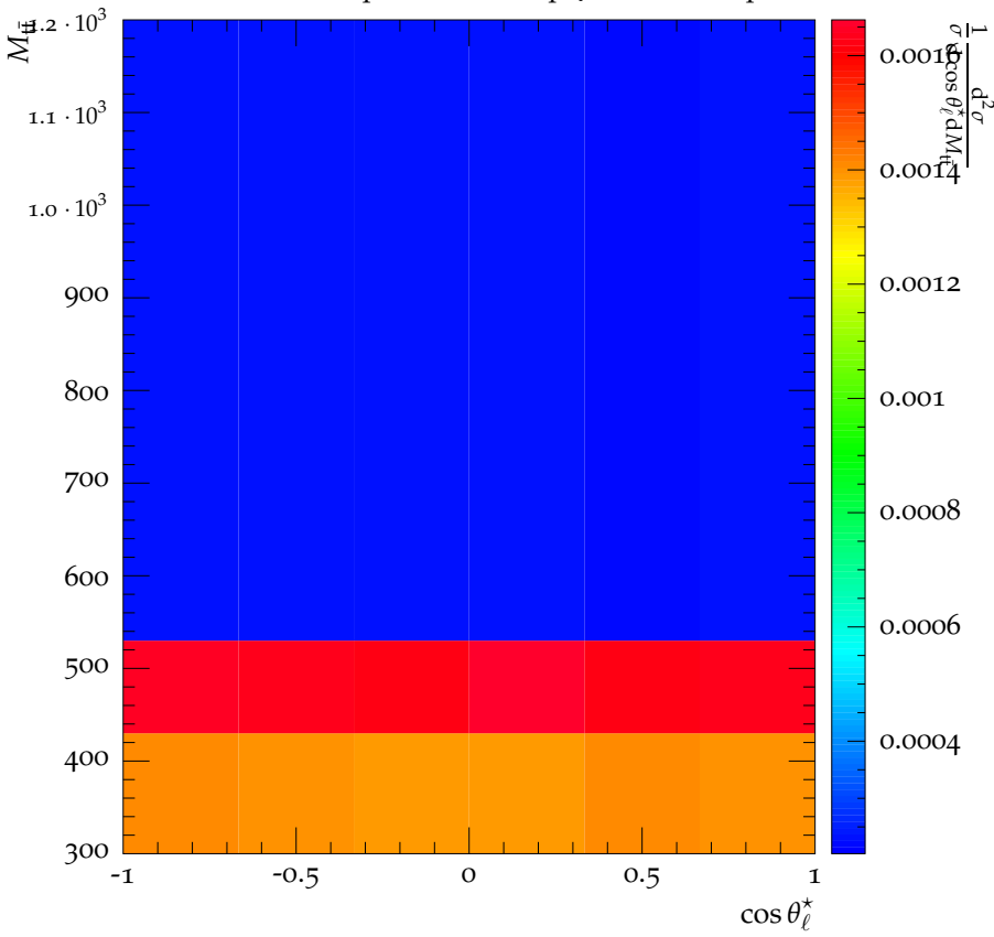
CMS, 8 TeV, t\bar{t} dilepton channel, H \rightarrow \gamma\gamma NLO Dipoles
