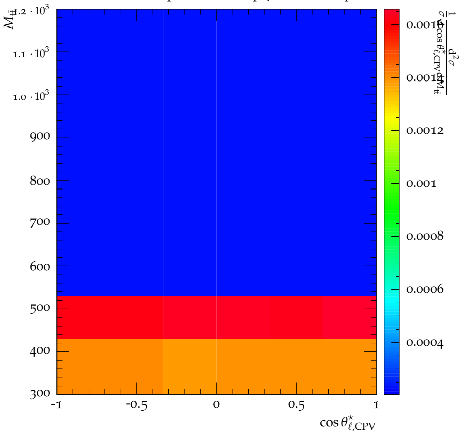
CMS, 8 TeV, t\bar{t} dilepton channel, Higgs to NLO Dipoles
