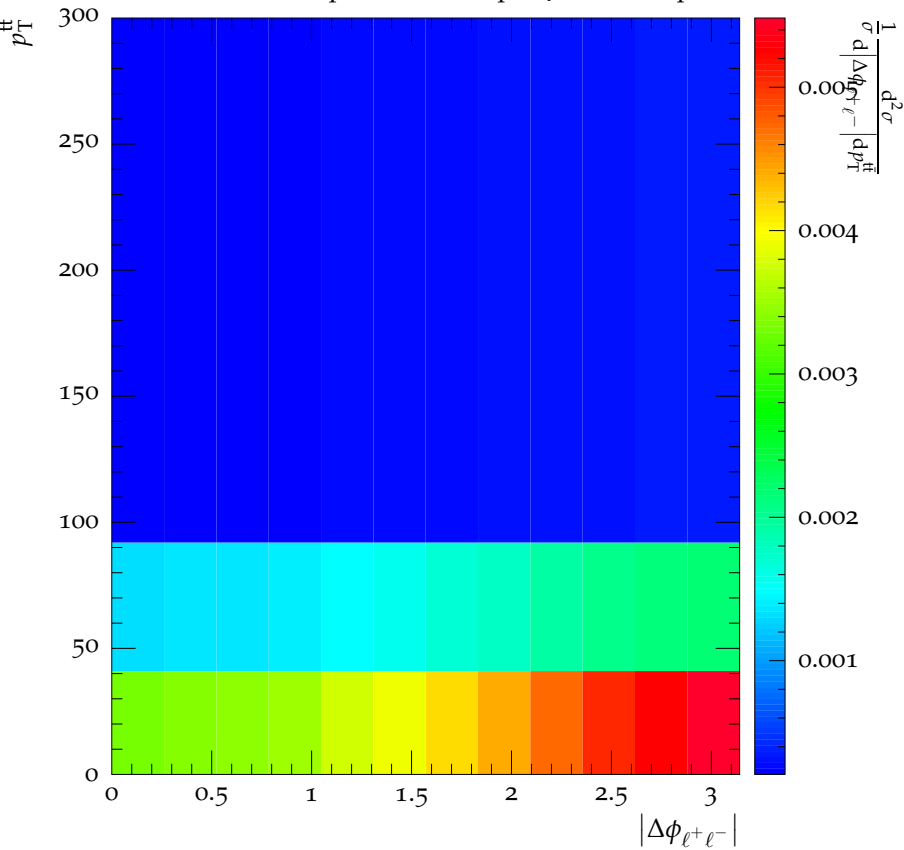
CMS, 8 TeV, t\bar{t} dilepton channel, \mu on Level Dipoles
