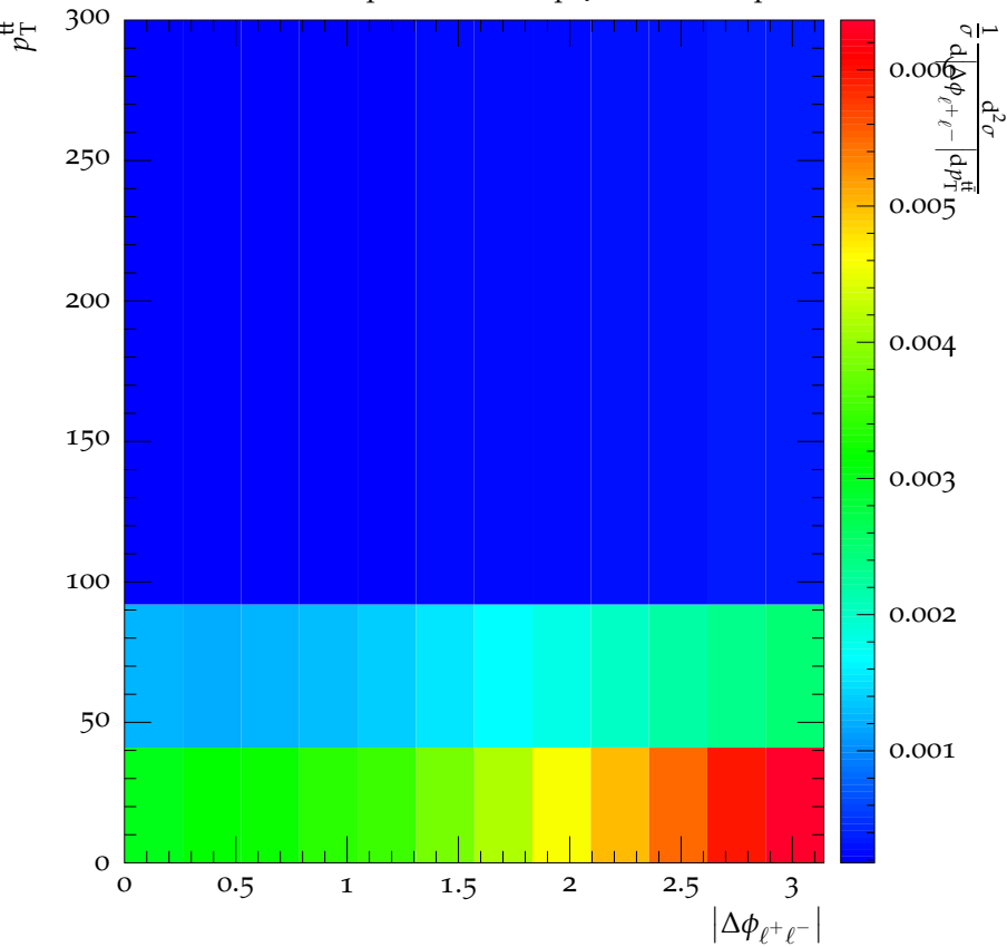
CMS, 8 TeV, t\bar{t} dilepton channel, H, \gamma Z, NLO, Dipole
