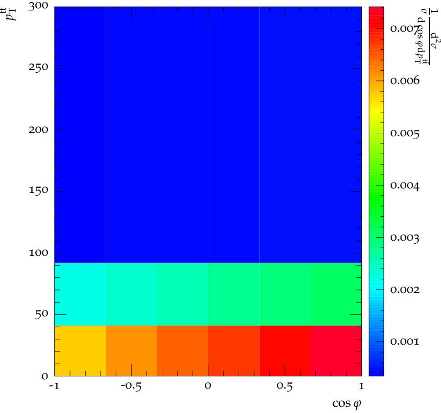
CMS, 8 TeV, t\bar{t} dilepton channel, \sqrt{s} = 1.0 TeV, Dipoles
