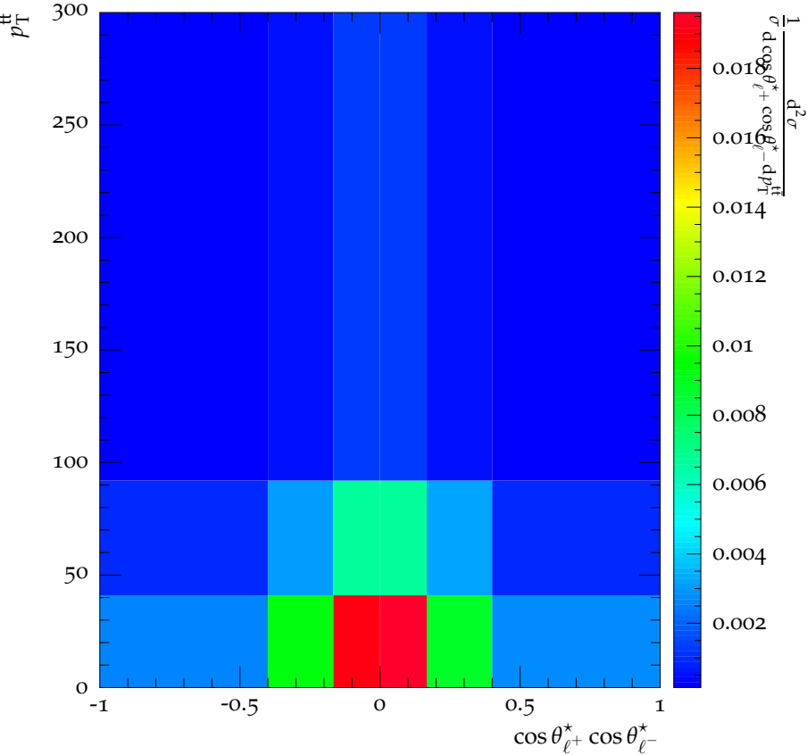
CMS, 8 TeV, t\bar{t} dilepton channel, parton-level \sigma \times \frac{1}{d^2\sigma} Merging
