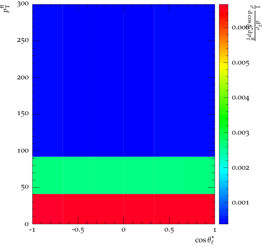
CMS, 8 TeV, t\bar{t} dilepton channel, \sqrt{s} = 1.96 TeV, Level 1 Dipoles
