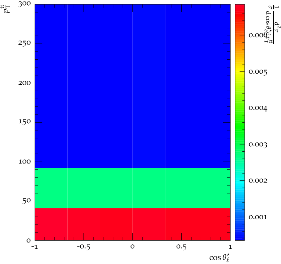
CMS, 8 TeV, t\bar{t} dilepton channel, \mu = 100 GeV, NLO, Dipole
