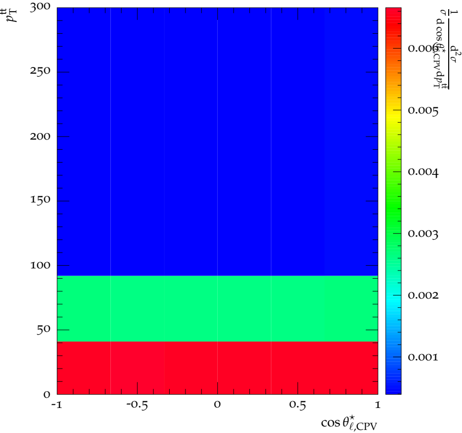
CMS, 8 TeV, t\bar{t} dilepton channel, \mu\mu or e\bar{e} Dipoles
