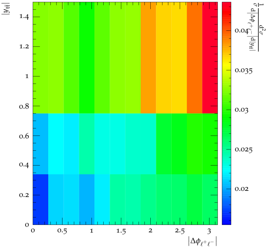
CMS, 8 TeV, t\bar{t} dilepton channel, parton-level Data
