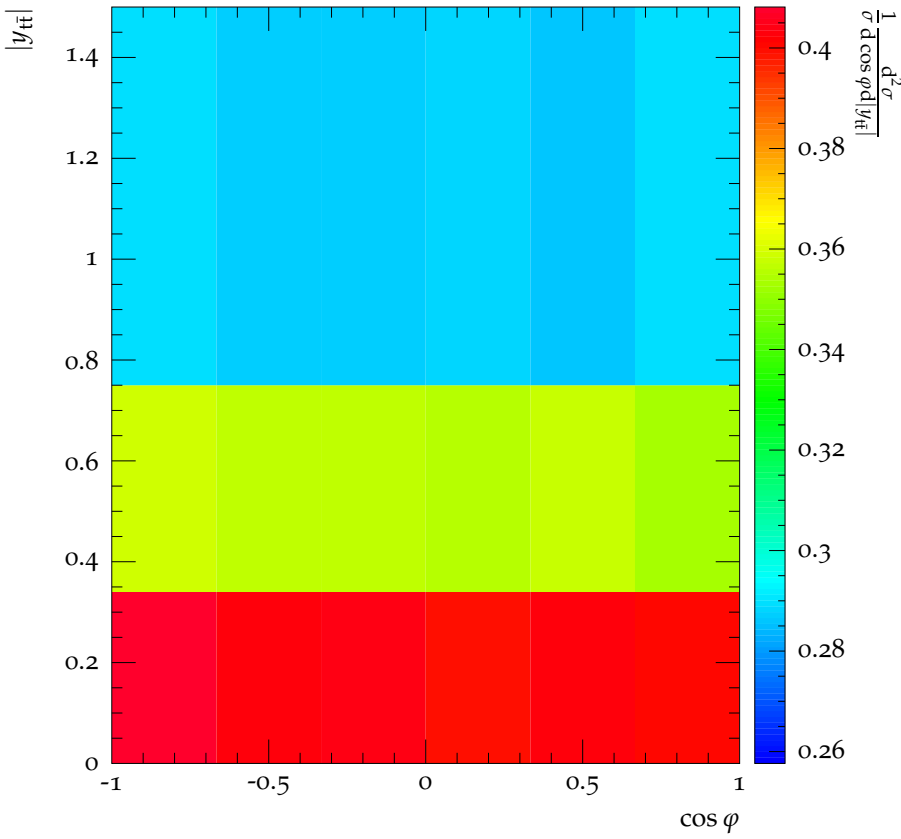
CMS, 8 TeV, t\bar{t} dilepton channel, H \rightarrow \gamma\gamma NLO \oplus Dipoles
