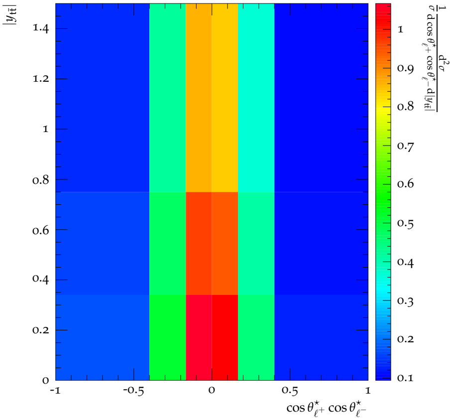
CMS, 8 TeV, t\bar{t} dilepton channel, \text{H} \rightarrow \gamma\gamma Dipoles
