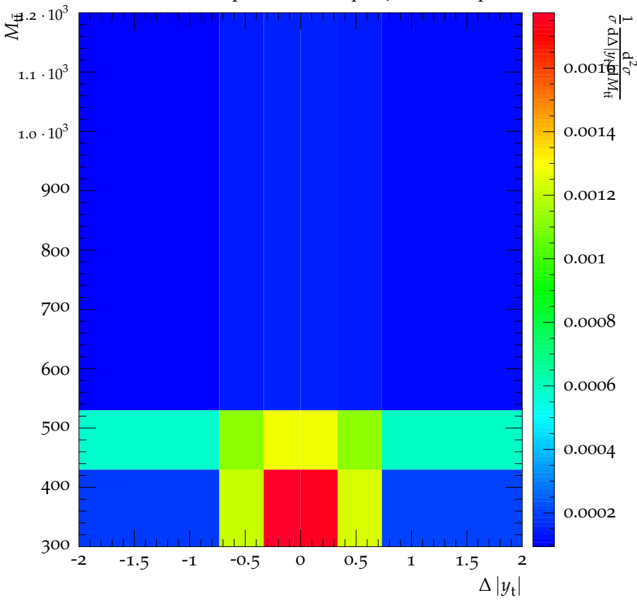
CMS, 8 TeV, t\bar{t} dilepton channel, \mu = 100 GeV, \sigma_{\text{Higgs}} \sim 1.5 \text{ fb} , Dipoles
