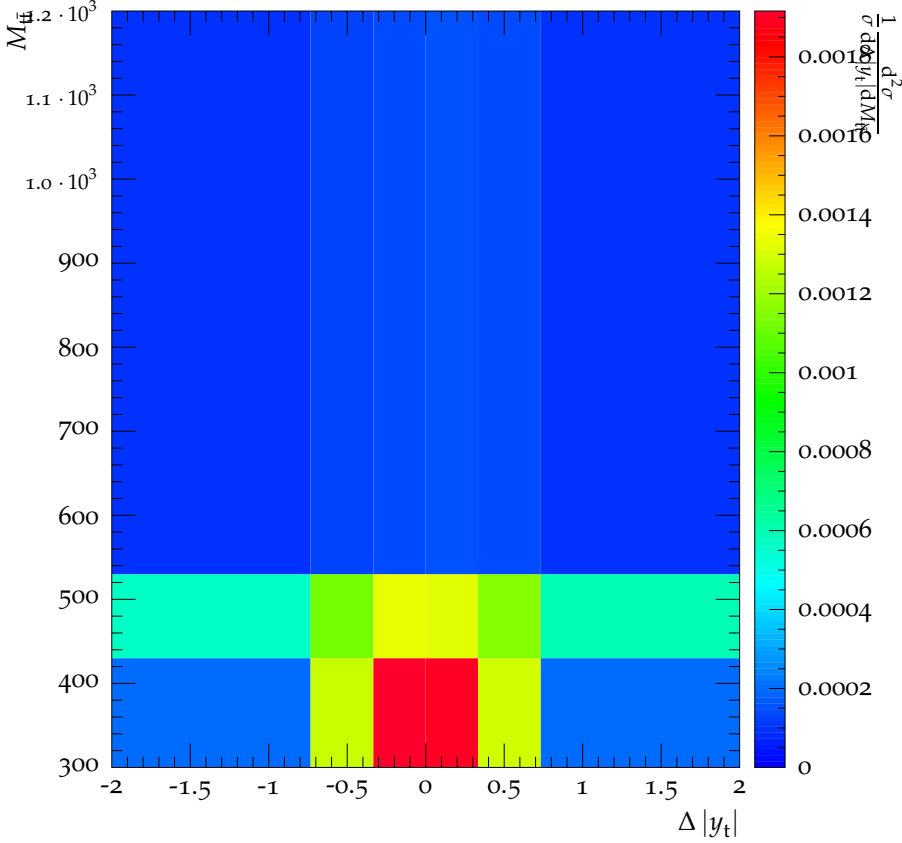
CMS, 8 TeV, t\bar{t} dilepton channel, \mu = 100 GeV, NLO Dipoles
