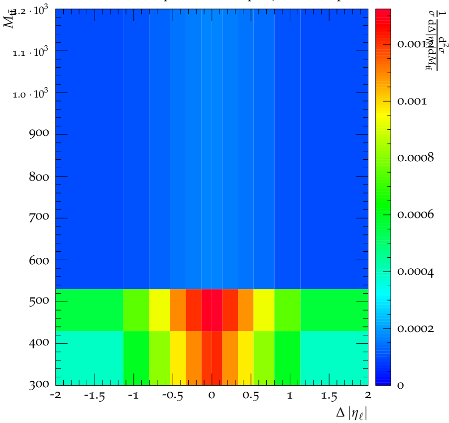
CMS, 8 TeV, t\bar{t} dilepton channel, H to \gamma\gamma Dipoles
