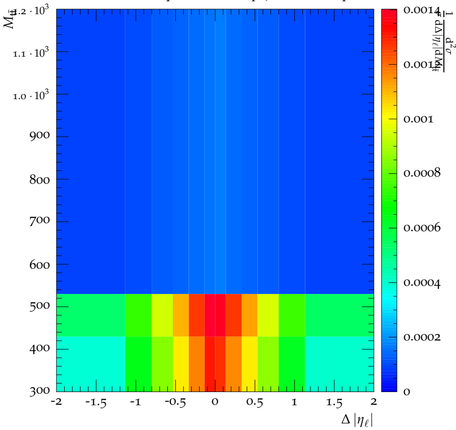
CMS, 8 TeV, t\bar{t} dilepton channel, \mu variation, Level 1 Dipoles
