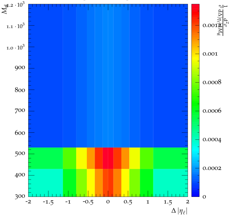
CMS, 8 TeV, t\bar{t} dilepton channel, parton level LO \oplus PS
