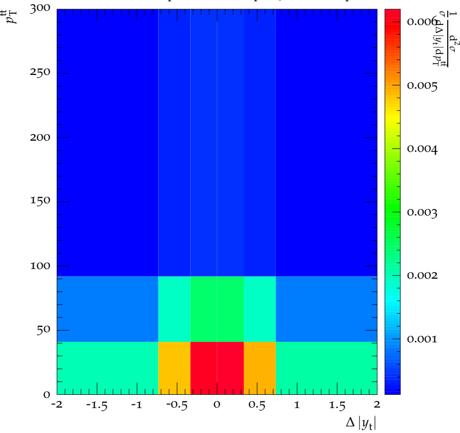
CMS, 8 TeV, t\bar{t} dilepton channel, \sqrt{s} = 1.96 TeV, Dipoles
