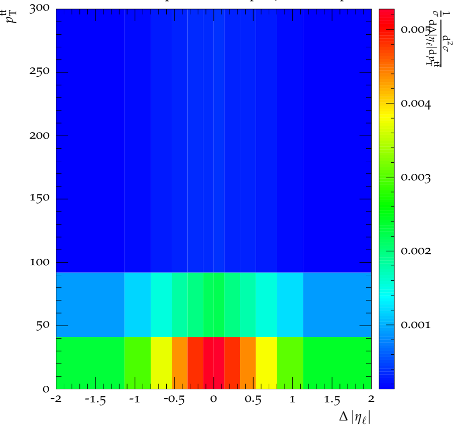
CMS, 8 TeV, t\bar{t} dilepton channel, \mu = 100 GeV, \sigma_{t\bar{t}} = 0.1 pb, \sigma_{\text{dipole}} = 0.1 pb
