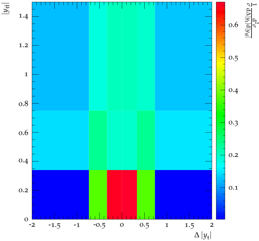
CMS, 8 TeV, t\bar{t} dilepton channel, \text{Harton Level 1} \oplus Dipoles
