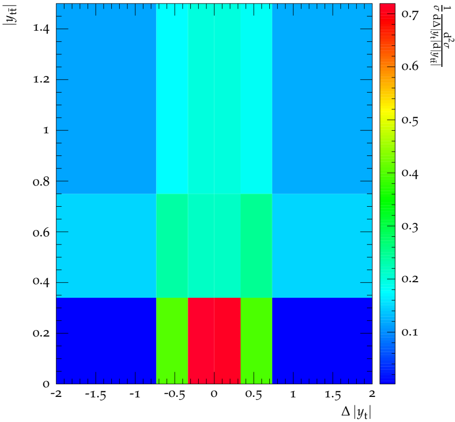
CMS, 8 TeV, t\bar{t} dilepton channel, \mu = 100 GeV, \sigma_{\text{H} \rightarrow \text{ZZ}}^{\text{NLO}} Dipoles
