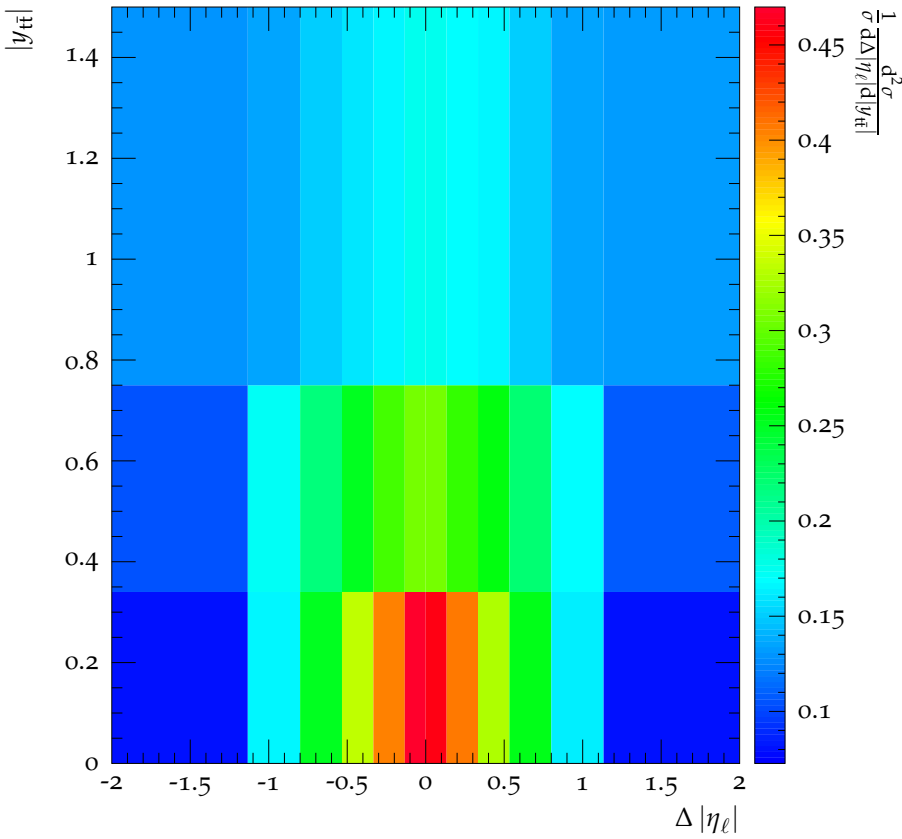
CMS, 8 TeV, t\bar{t} dilepton channel, H, \gamma or Z level Dipoles
