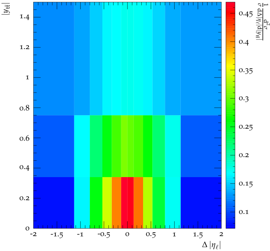
CMS, 8 TeV, t\bar{t} dilepton channel, parton-level NLO \oplus PS
