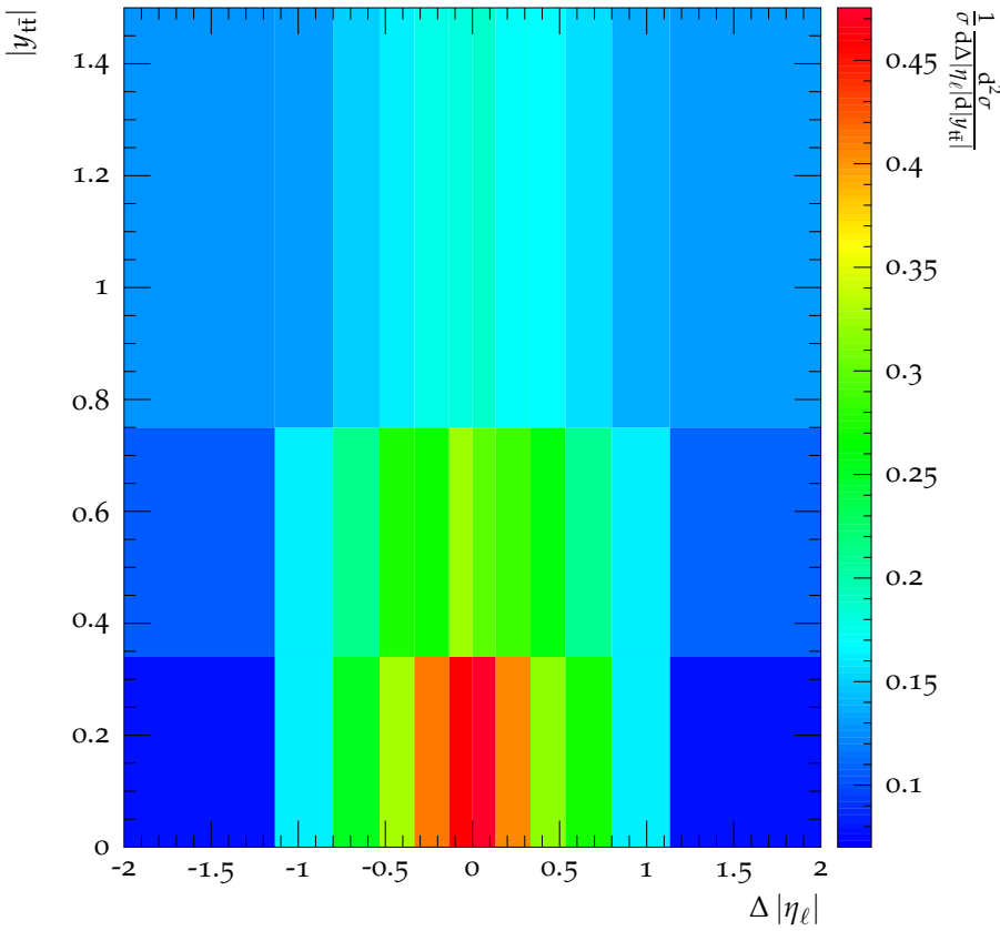
CMS, 8 TeV, t\bar{t} dilepton channel, parton-level merging
