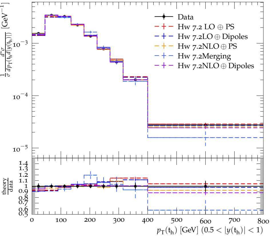
CMS, 13 TeV, t\bar{t} lepton+jets
