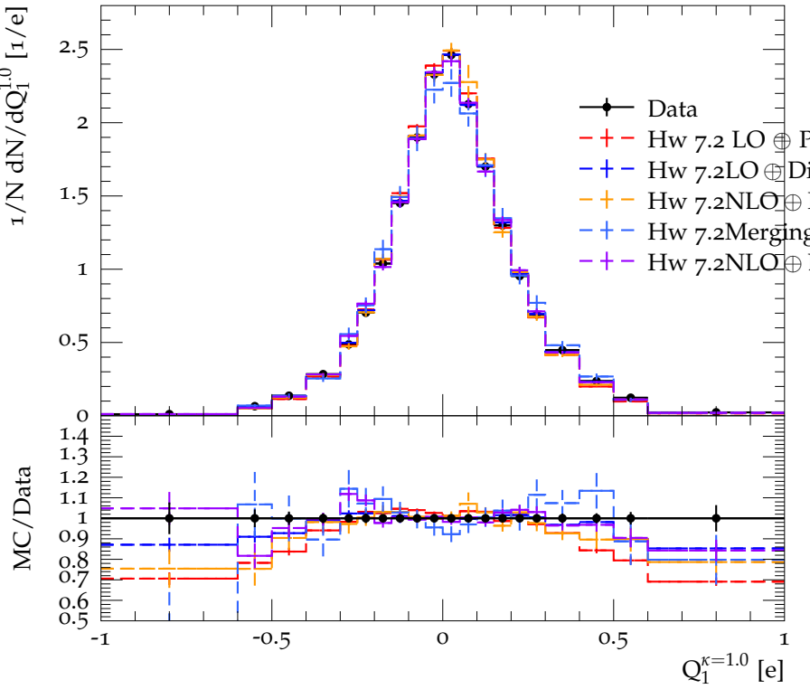
CMS, 8 TeV, jetcharge of leading jet ( p_T > 400 GeV, \eta < 1.5 )
