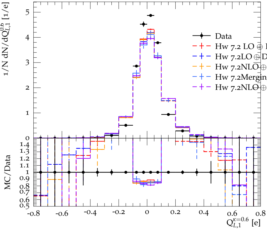
CMS, 8 TeV, jetcharge of leading jet ( 700 < p_T < 1000 GeV, \eta < 1.5 )
