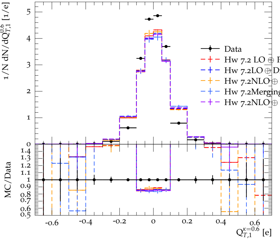
CMS, 8 TeV, jetcharge of leading jet ( 400 < p_T < 700 GeV, \eta < 1.5 )
