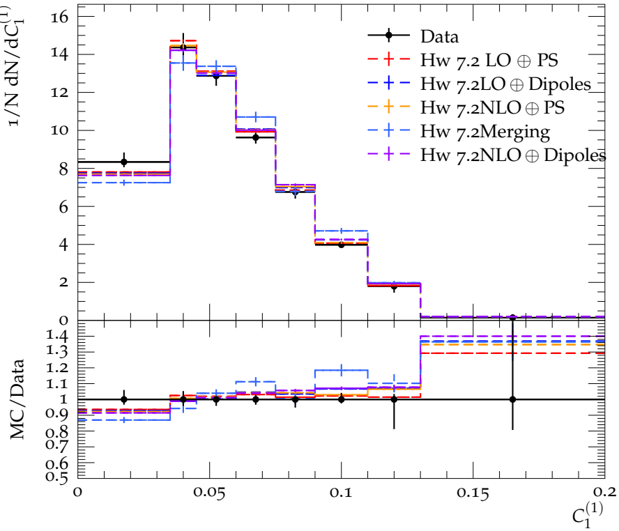
CMS, 13 TeV, t\bar{t} lepton+jets, incl jets, charged particles
